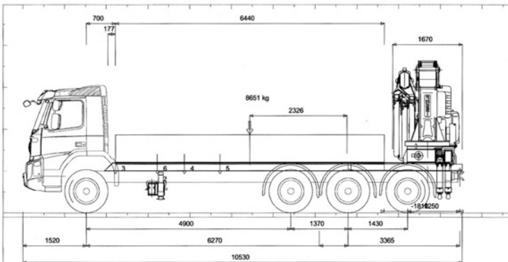
VOLVO FMX 500 8x4 FASSI F710RA.2.26
